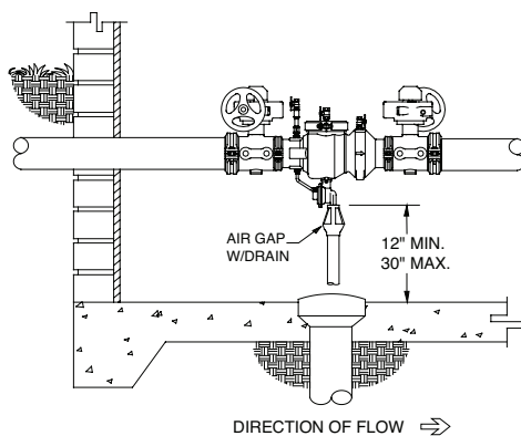
INDOOR INSTALLATION (375A with BG option)
